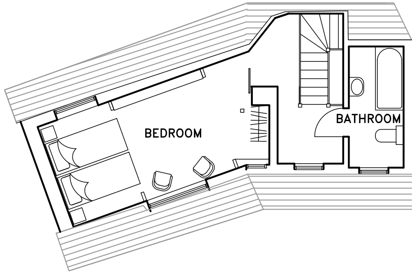
BAY COTTAGE FIRST FLOOR
